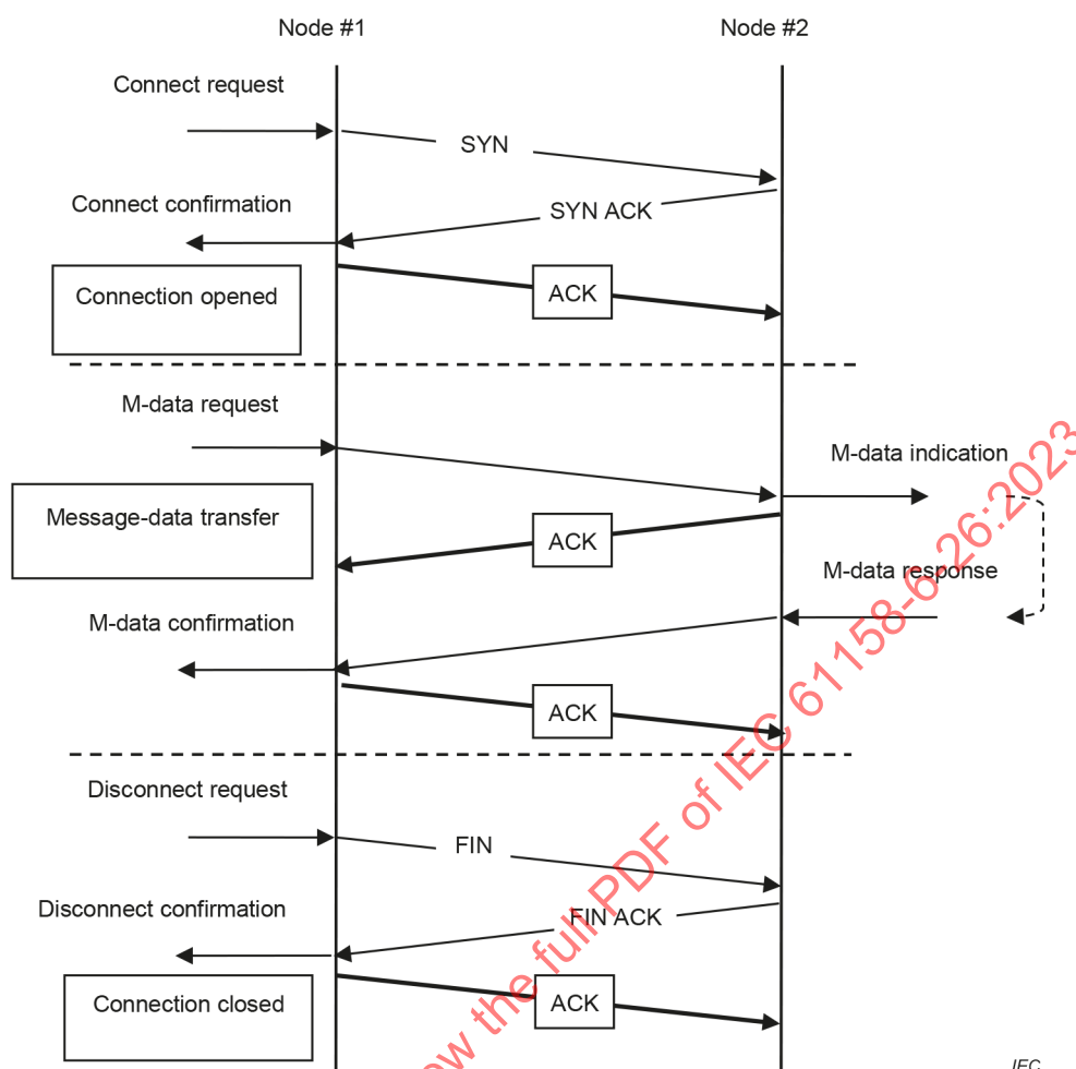
Figure 16 – Delivery confirmation checked by TCP protocol
