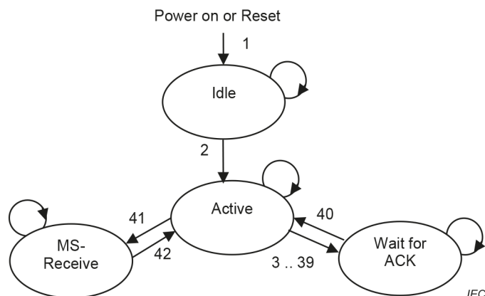
Figure 60 – State transition diagram of Message-data protocol machine
