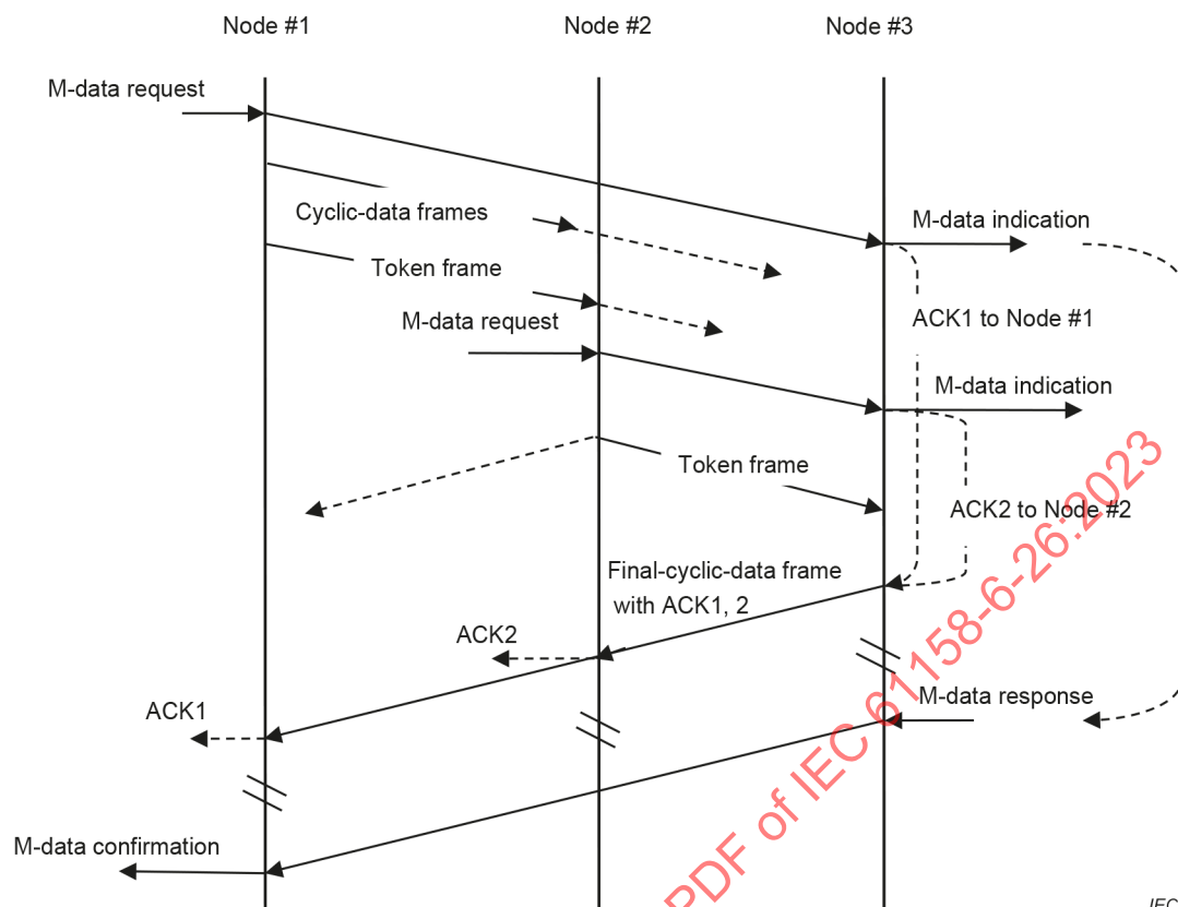
Figure 15 – Example of sequential diagram of ACK over UDP channel
