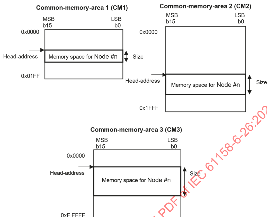
Figure 12 – Configuration of the Common-memory
