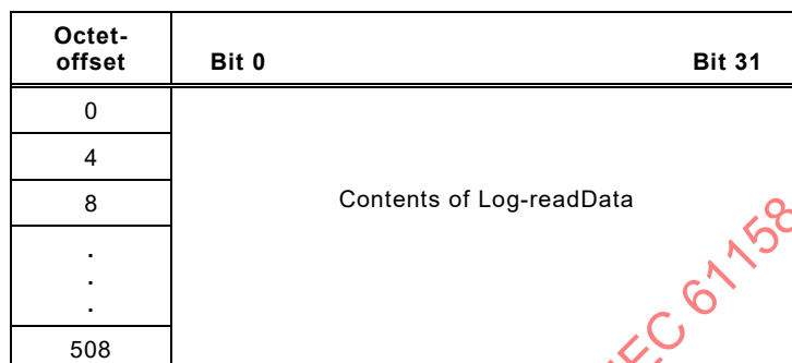
Figure 36 – Structure of Log-readData with M_RLT = 0
