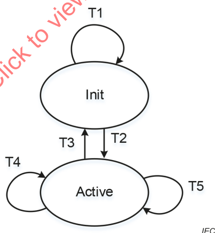
Figure 10 – Diagram of transition state of ALCE state machine
