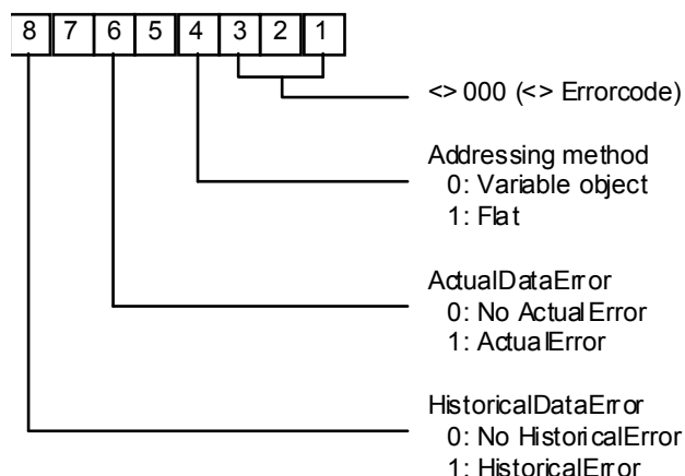
Figure 5 – Remaining subfields of ControlStatus
