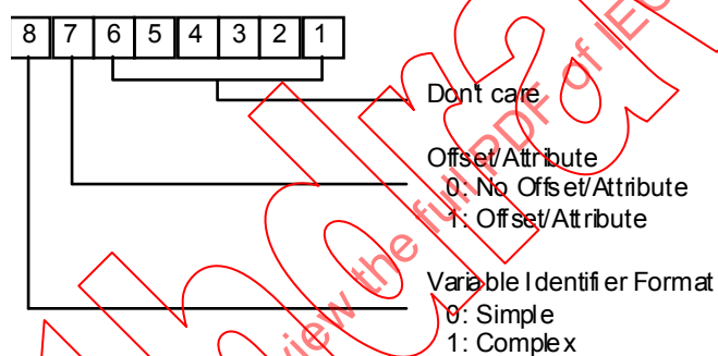
Figure 6 – DataFieldFormat encoding
