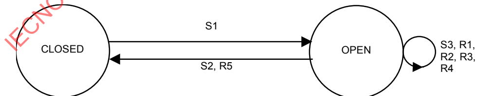
Figure 3 – State transition diagram of the publisher / subscriber ARPM
