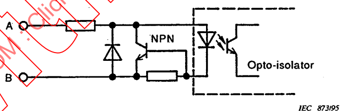
Figure 4 – Example 2, opto-isolator based listener circuit
