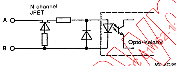
Figure 3 – Example 1, opto-isolator based listener circuit
