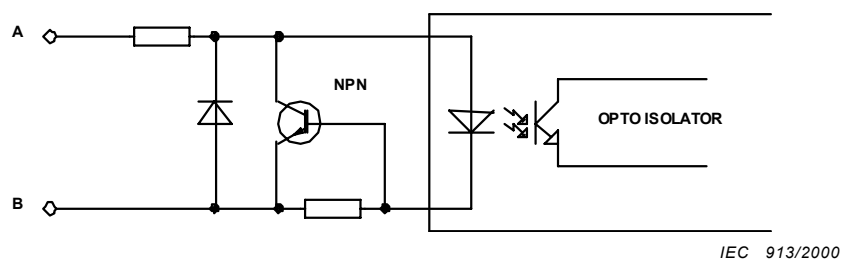
Figure 4 – Example 2, NPN opto-isolator based listener circuit
