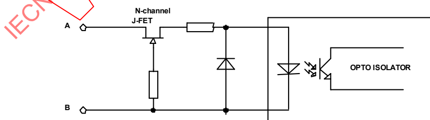
Figure 3 – Example 1, J-FET, N channel, opto-isolator based listener circuit
