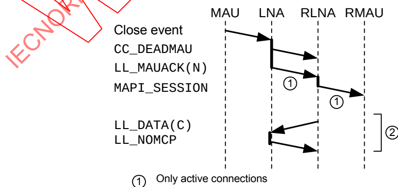
Figure 22 – Closing a MAU connection
