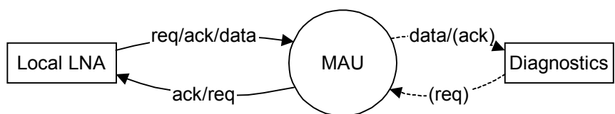
Figure 2 – MAU context diagram
