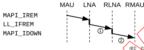
Figure 26 – Closing accept interface
