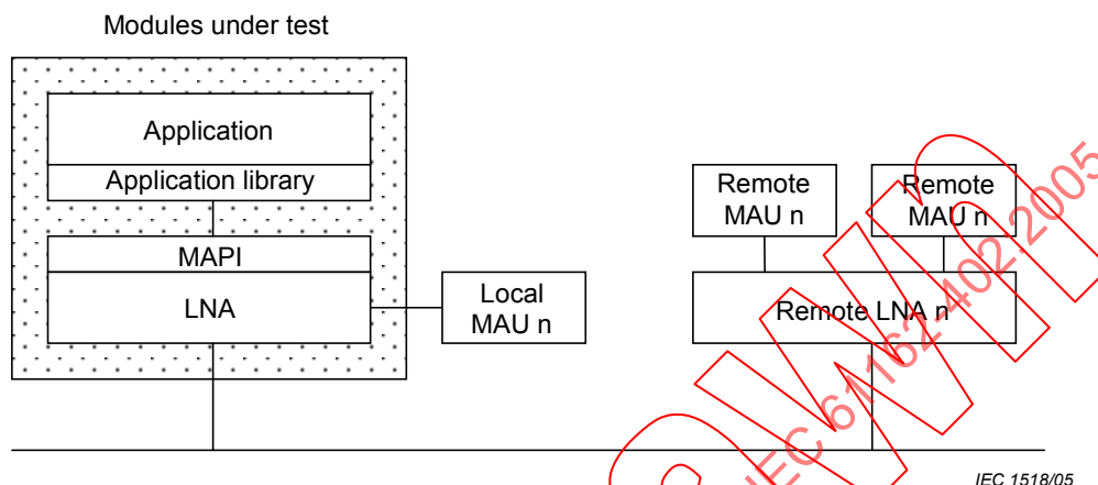
Figure 3 – Test topology
