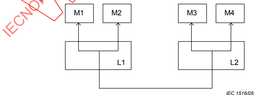
Figure 1 – Typical communication paths in an IEC 61162-4 system
