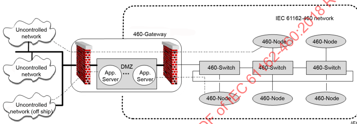
Figure 2 – 460-Network with 460-Gateway
