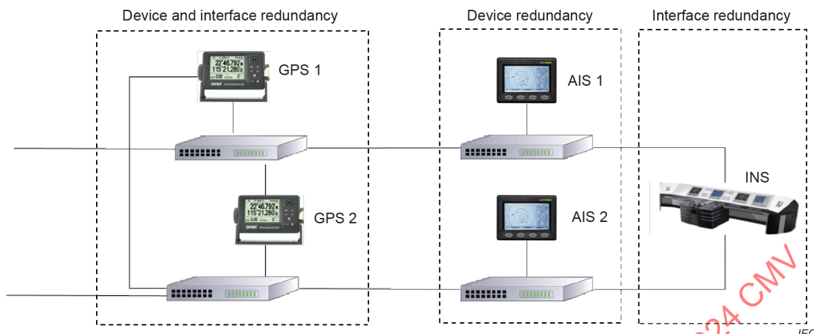
Figure 3 – Example of redundancy
