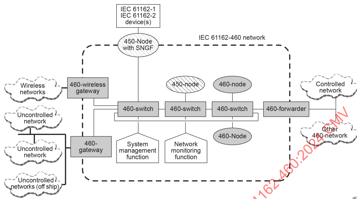
Figure 1 – Functional overview of IEC 61162-460 requirement applications
