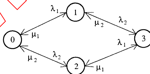
Figure 9 – State-transition diagram for a two-unit system with restorable units
