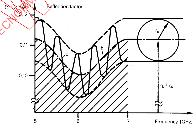
Figure 6c – Extraction of r_c (ripple E) by dividing the difference r_{\max} - r_{\min} by 2. r_c is the reflection factor of the connector under test (including the reflection of the standard test connector at C in figure 4)
