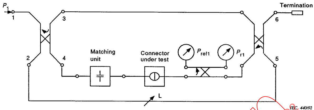
Figure 13 – Ring line method with variable coupling
