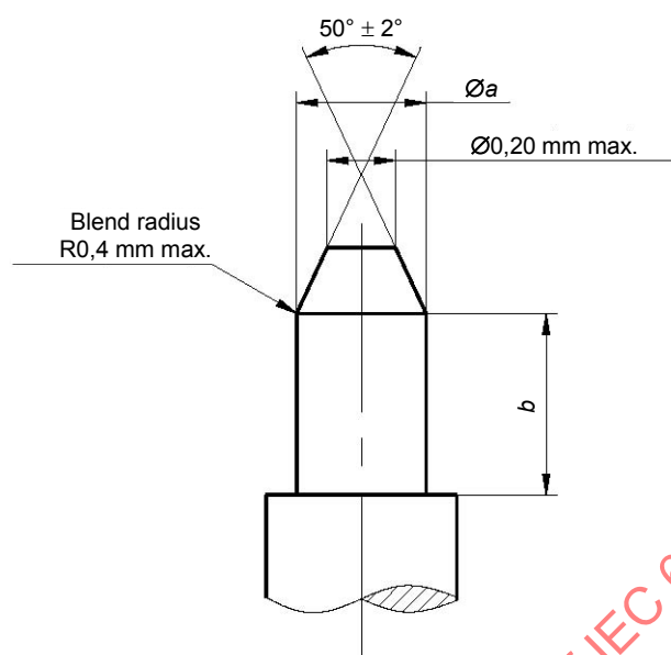
Figure 3 – Gauge pins for socket-centre contact (for dimensions and notes, see Table 3)
