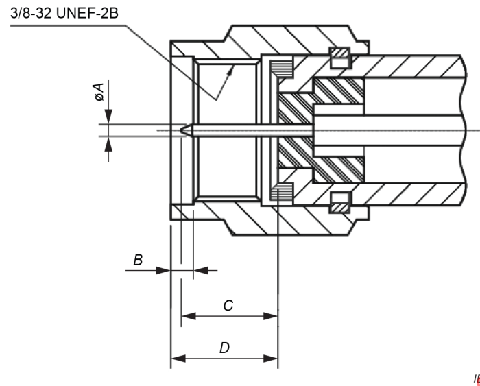
Figure B.2 – Satellite broadcasting “F” type male plug (for dimensions, see Table B.2)
