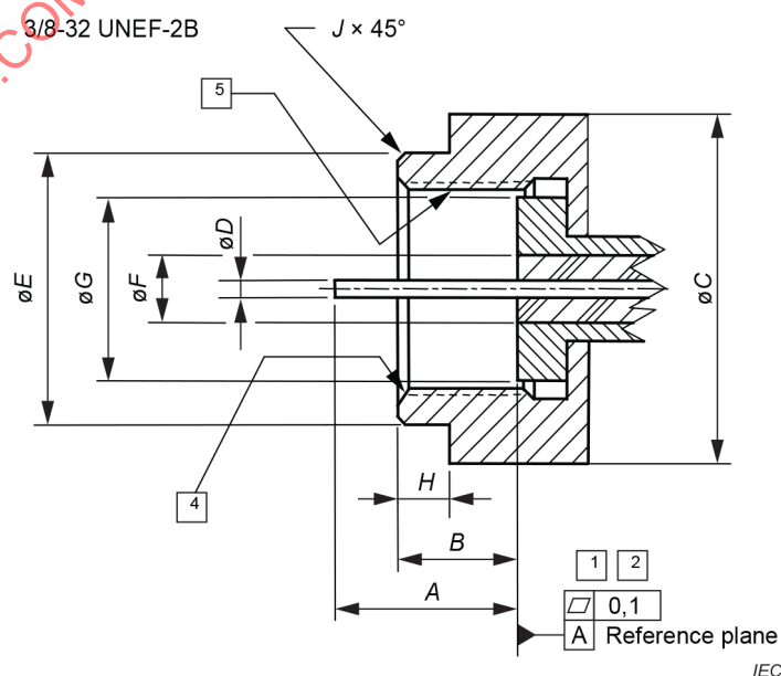
Figure A.2 – Outdoor “F” type male plug (for dimensions, see Table A.2)
