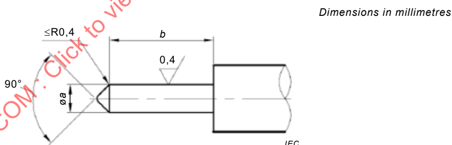
Figure 3 – Gauge pin for socket-centre contact (for dimensions, see Table 3)
