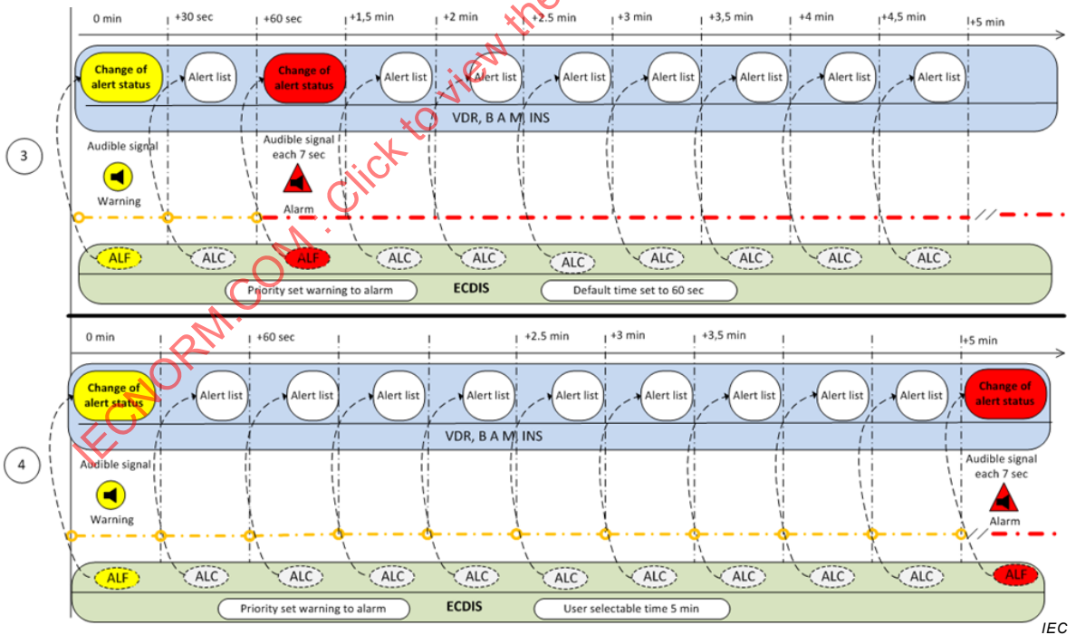
Figure Q.3 – Alert reporting by ECDIS with escalation of a warning as alarm
