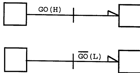
Figure 12 - Mismatched polarity indications
