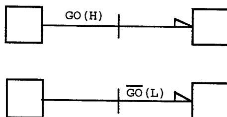
Figure 12 - Indications de polarité non assorties
