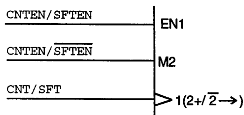
Figure 9 - Example of signal names for multifunction signals
