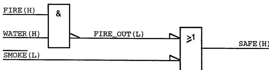
Figure 11 - Polarity indications and signal levels
