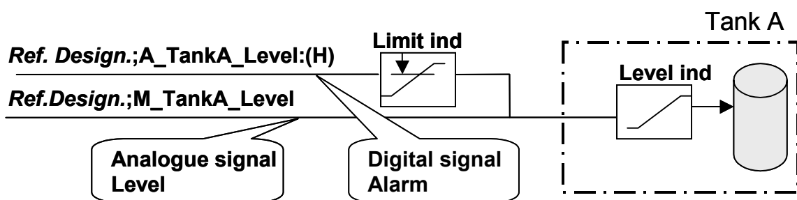
Figure 8 – Example of parts of an analogue signal
