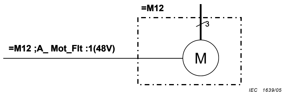
Figure 21 – Example of signal designation corresponding to conformance class 2
