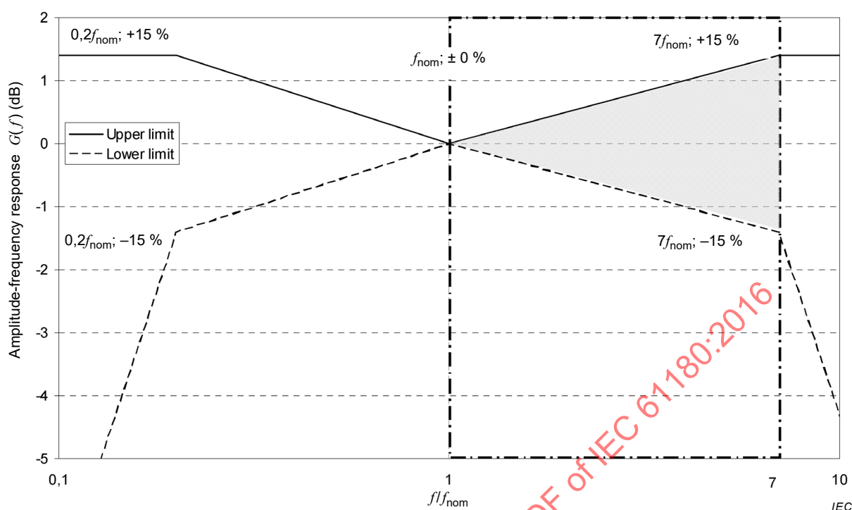
Figure 4 – Shaded area for acceptable normalised amplitude-frequency responses of measuring systems intended for single fundamental frequencies f_{\text{nom}} (to be tested in the range (1 \dots 7) f_{\text{nom}} )
