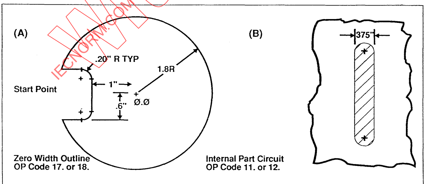
Figure 8-3 – Part outlines
