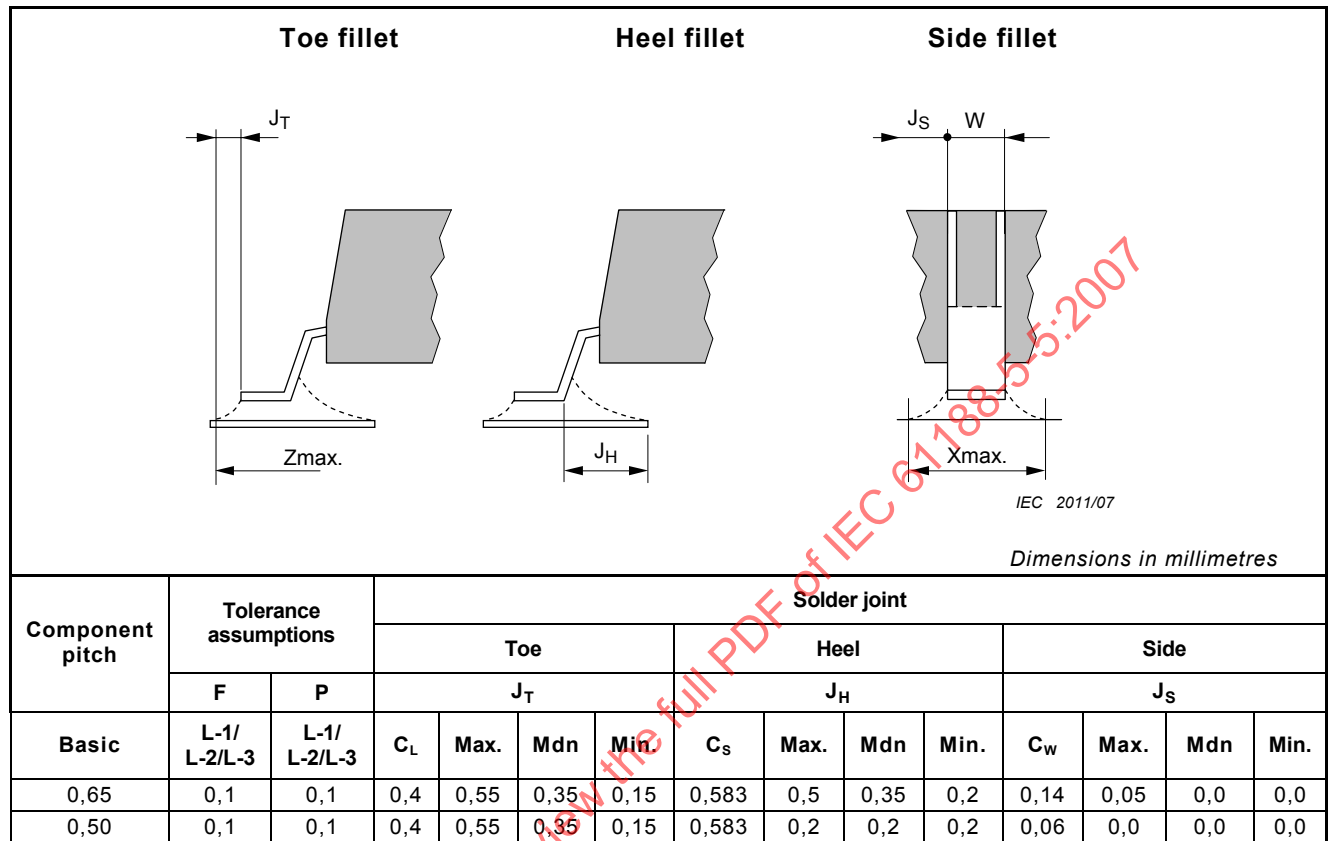
Figure 15 – Solder joint fillet design
