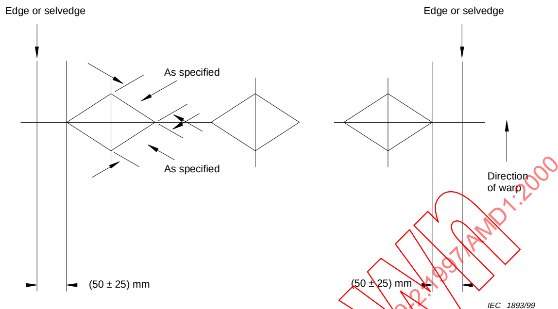
Figure 16 – Position of specimens for resin content
