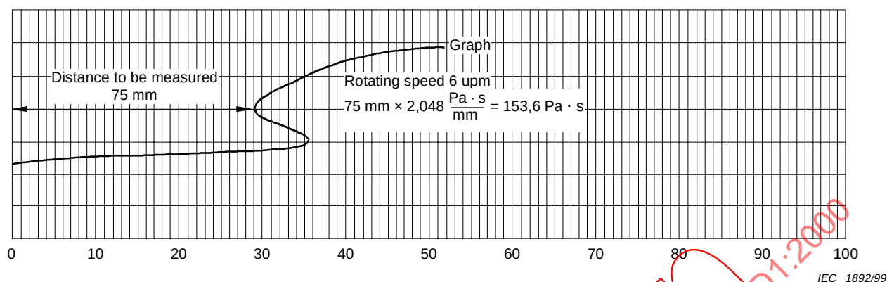
Figure 15 – Example of prepreg melting viscosity
