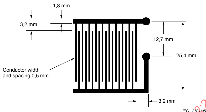
Figure 28 – Comb pattern
