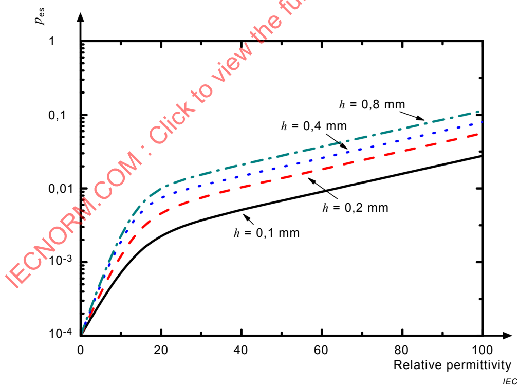
Figure B.4 – p_{es} versus relative permittivity at different sample thicknesses
