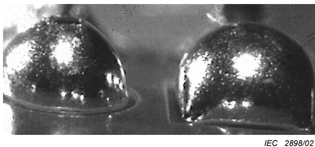
Figure 67 – Solder fillet – Nonconforming
