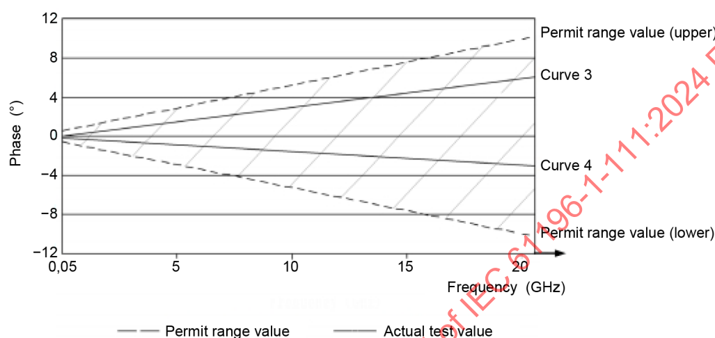
Figure 9 – Test graph schematic diagram
