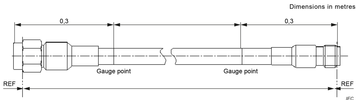
Figure A.1 – Preparation of TS for stability of attenuation constant
