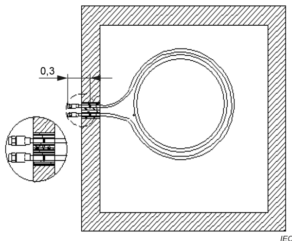
Figure A.2 – Schematic diagram of TS placement
