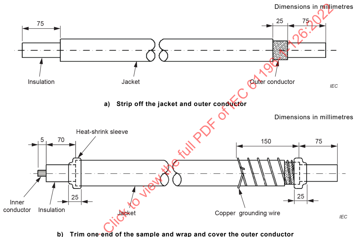
Figure 2 – Preparation of semi-flexible cable sample
