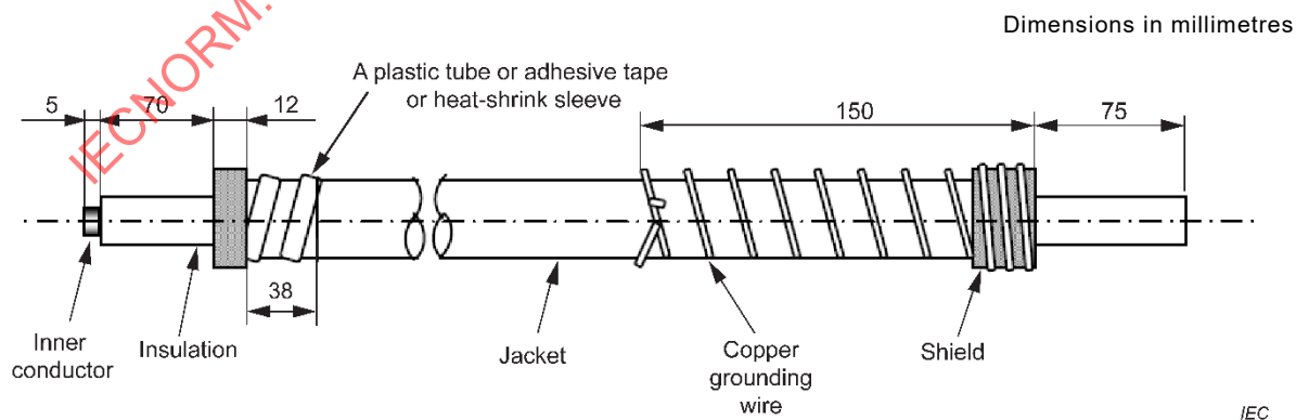
c) Trim one end of the sample and wrap the shield and jacket
