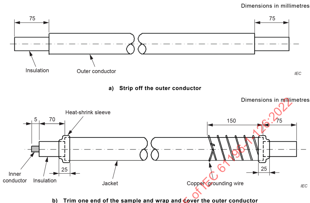
Figure 3 – Preparation of semi-rigid cable and unjacketed semi-flexible cable sample
