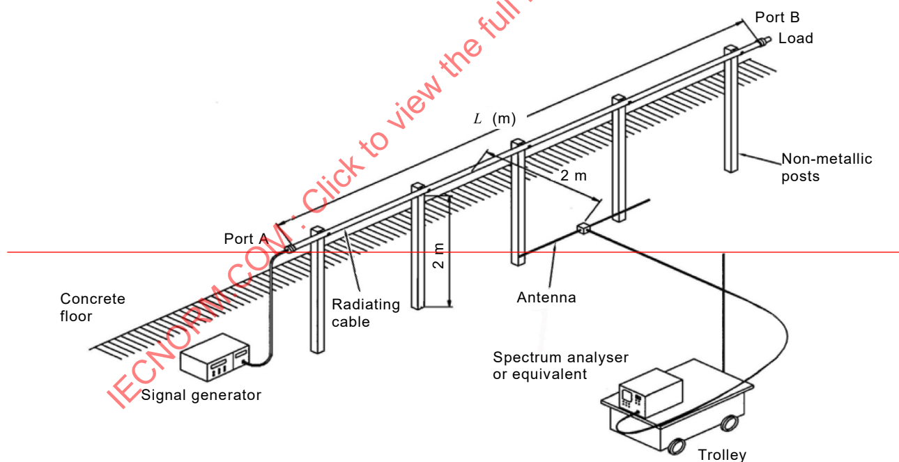
Figure B.3 — Coupling loss with ground-level method
