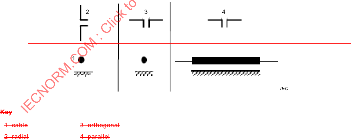
Figure B.1 Antenna orientations with ground-level method
