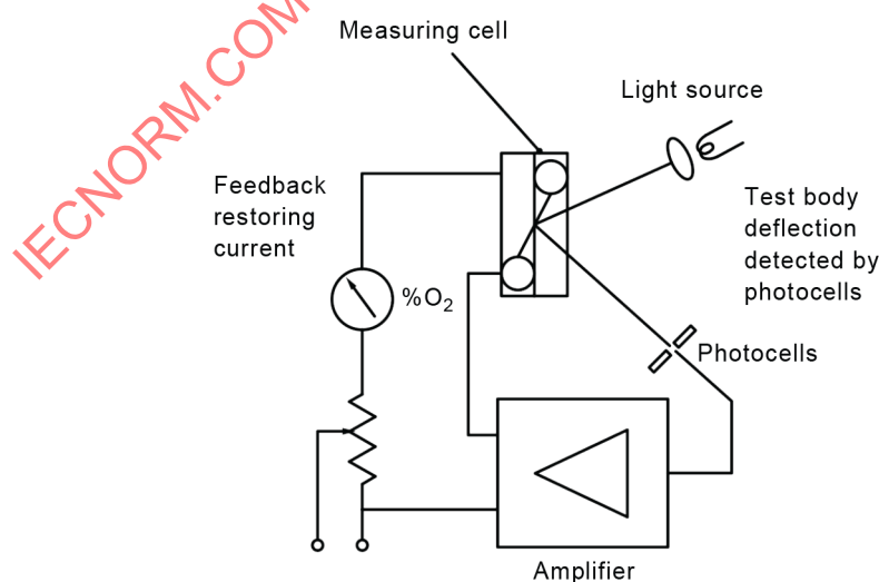
Figure 1 – Magnetic auto-balance system with current feedback
