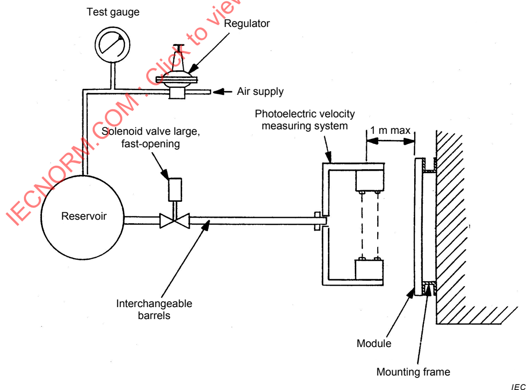
Figure 13 – Hail-test equipment
