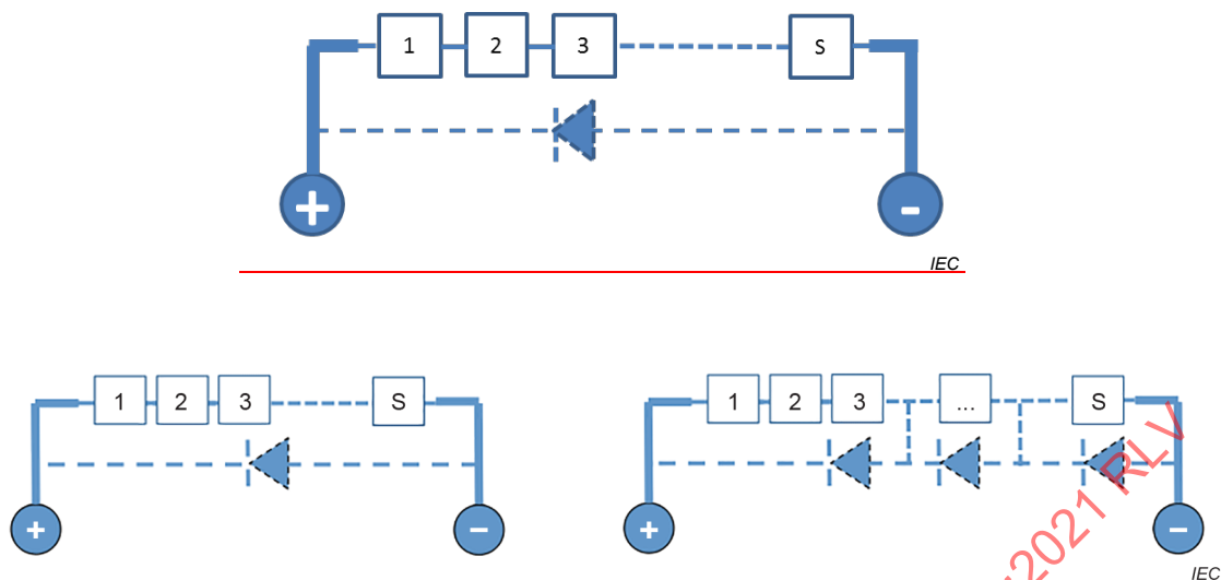
Figure 1 – Case S, series connection with optional bypass diode
