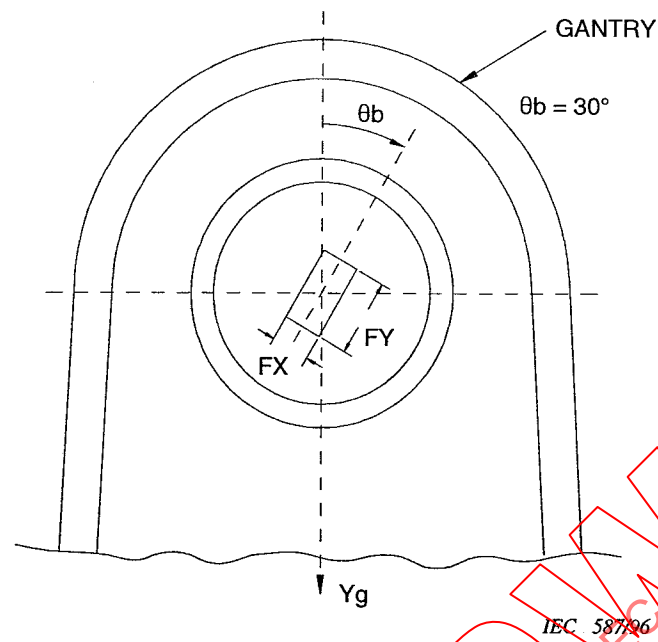
Figure 15a – Rotated ( \theta_b = 30^\circ ) symmetrical rectangular RADIATION FIELD (FX x FY) at NORMAL TREATMENT DISTANCE, viewed from ISOCENTRE looking toward RADIATION SOURCE (see 6.2)
