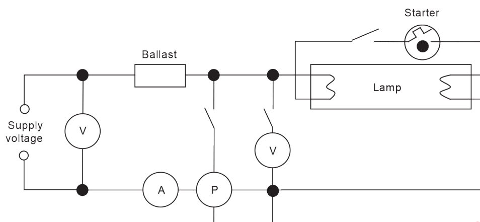
Figure 2 – Test circuit
