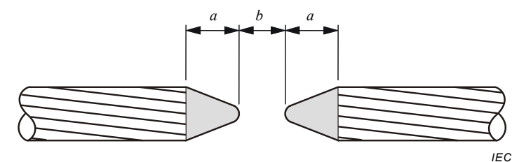
a) Ends prepared
