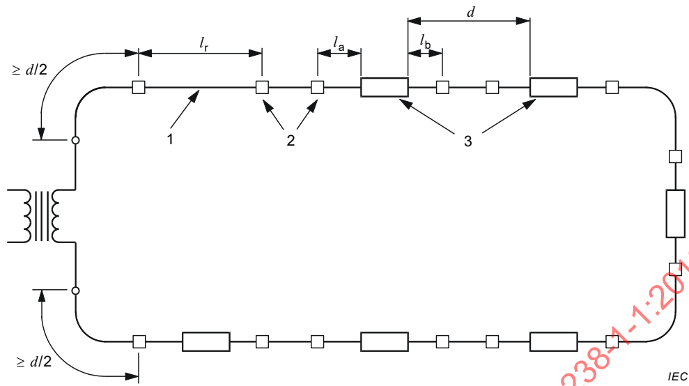
a) Through connectors – principle test loop
