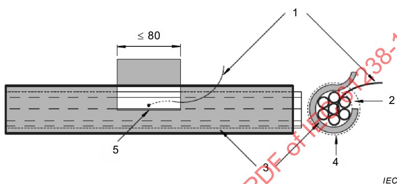
a) Position of thermocouple on stranded insulated reference cable
