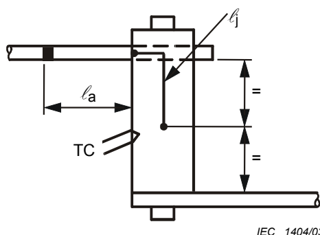
Figure 3g – Connection to the conductor for a mechanical connector
