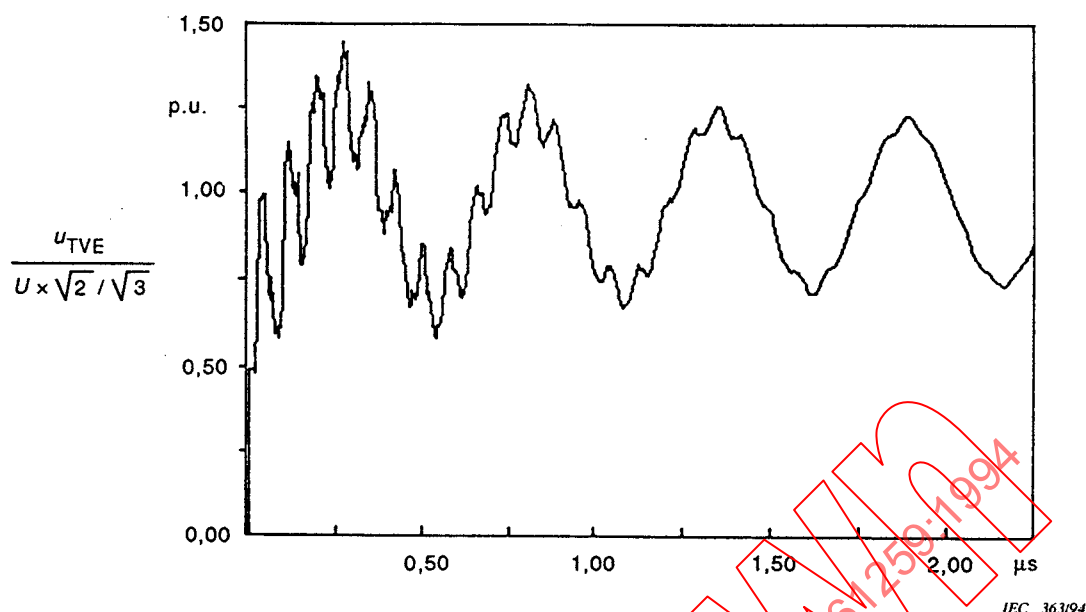
Figure 2 – Typical voltage wave-form (including VFT and FT components)
