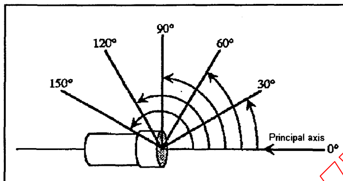
Figure 1 – Illustration of sound incidence angles from the principal axis of the microphone
