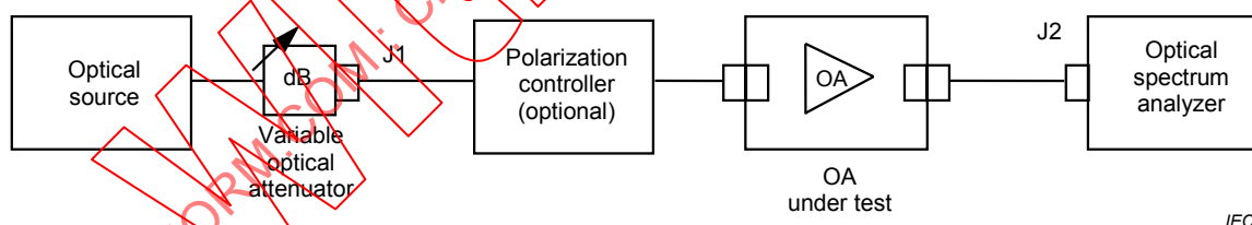
Figure 1b – Input signal power measurement
