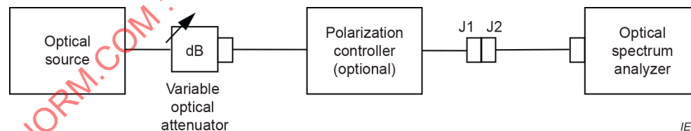
b) – Input signal power measurement
