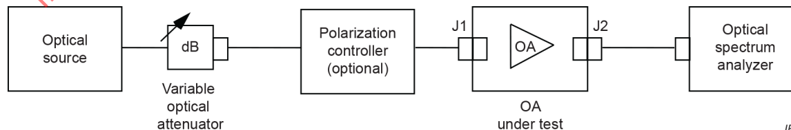
c) – Output power measurement
