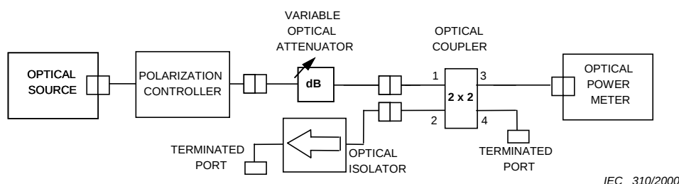
a) OFA input power measurement with optical power meter
