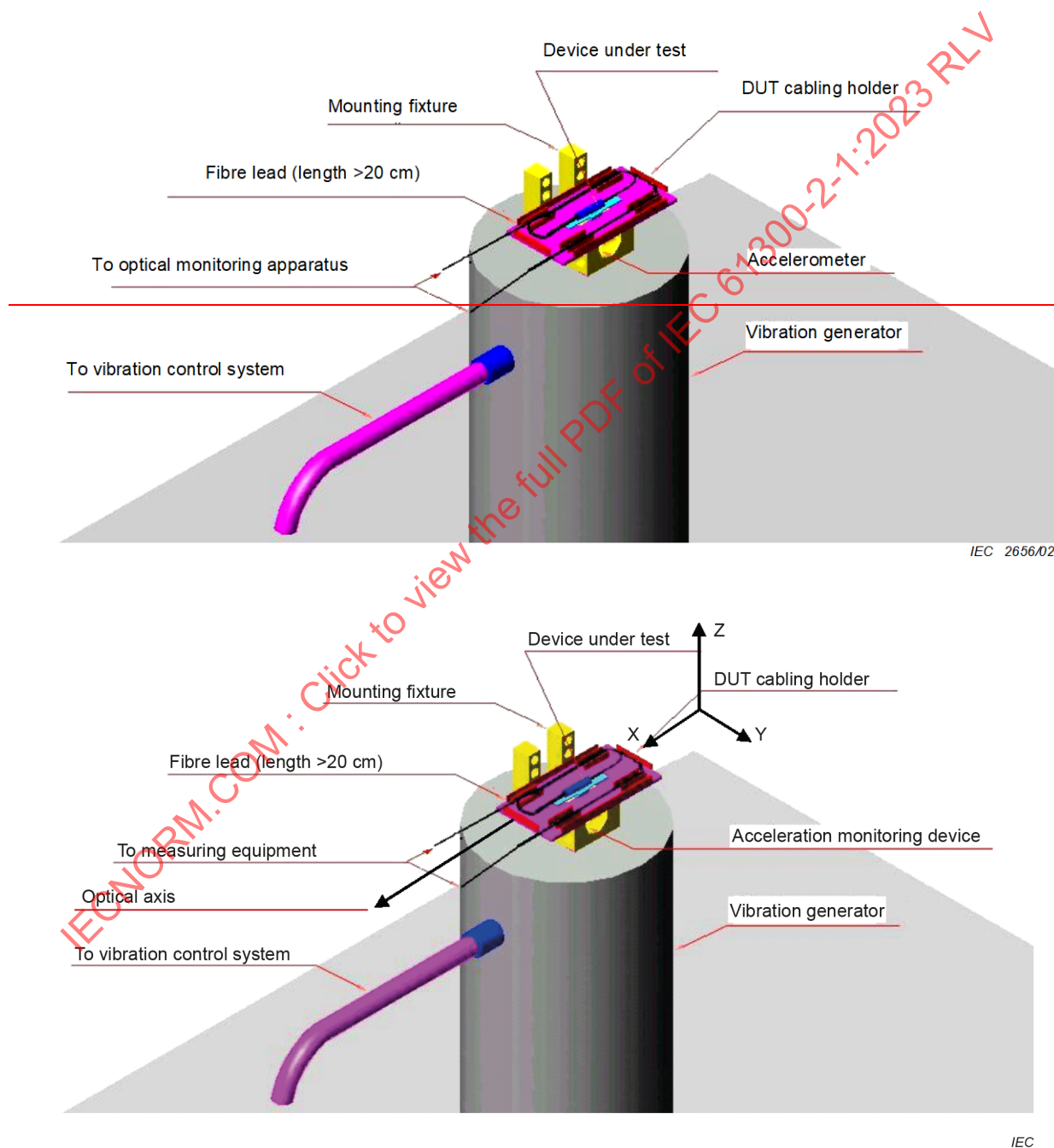
Figure 1 – Example of vibration apparatus
