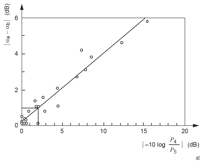
Figure A.5 – Relationship between power and \alpha
