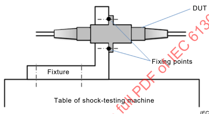
a) Fixing points using a fixture
