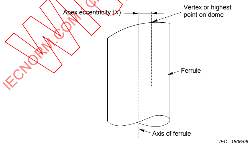
Figure 1 – Definition of apex eccentricity
