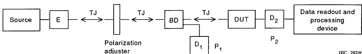
Figure 5 – Ratio measurement
