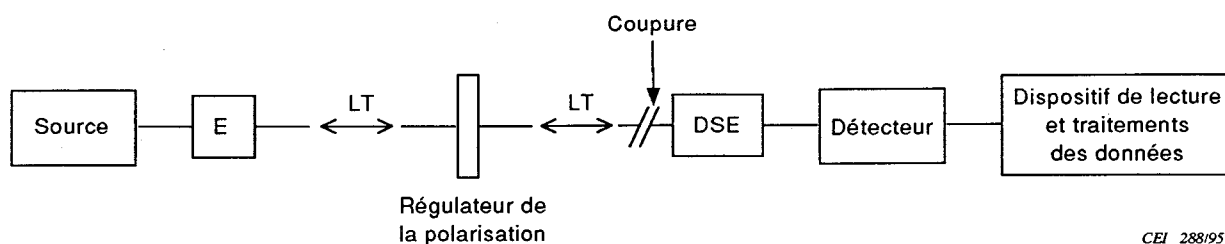
Figure 3b – Fibre coupée – phase 2
