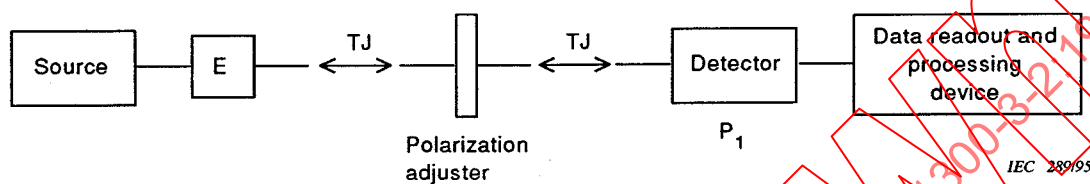
Figure 3c – Cutback – step 3
