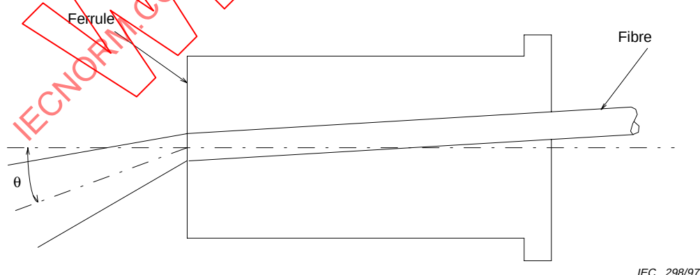
Figure 1 – Definition of angular misalignment
