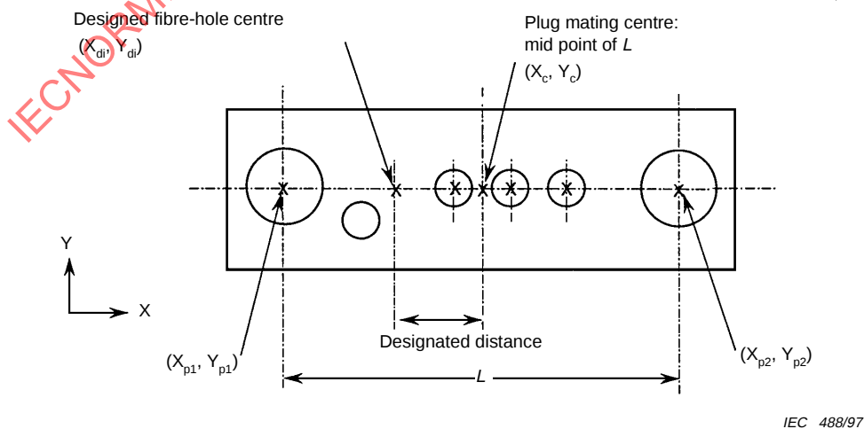
Figure 4 – Determination of intended fibre-hole centre
