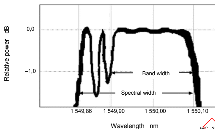
Figure 6 – BW and full spectral width for a fibre Bragg grating
